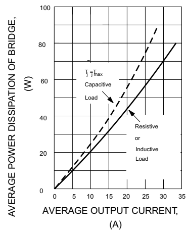
FIG.6-MAXIMUM POWER DISSIPATION
